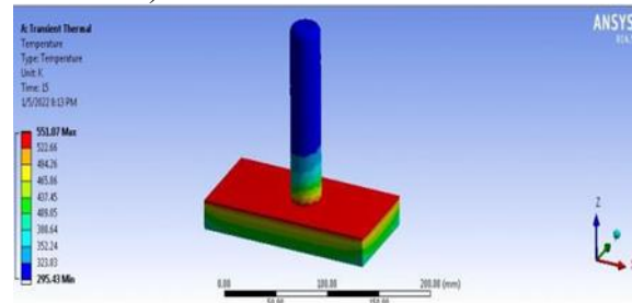
Fig 14: Temperature for Servo oil material
