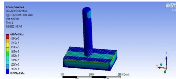
Fig 3: Strain at 3000 RPM for HSS material
