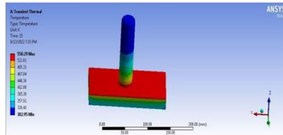
Fig 20: Temperature for palm oil material
