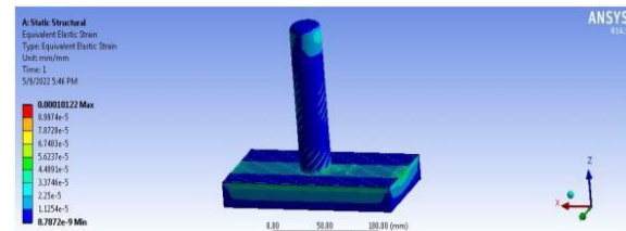
Fig 6: Strain at 3000 RPM for HSS material
