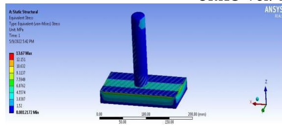
Fig 2: Stress at 3000 RPM for HSS material
