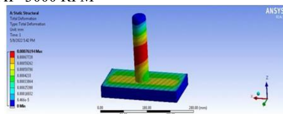
Fig 1: Total deformation at 3000 RPM for HSS material
